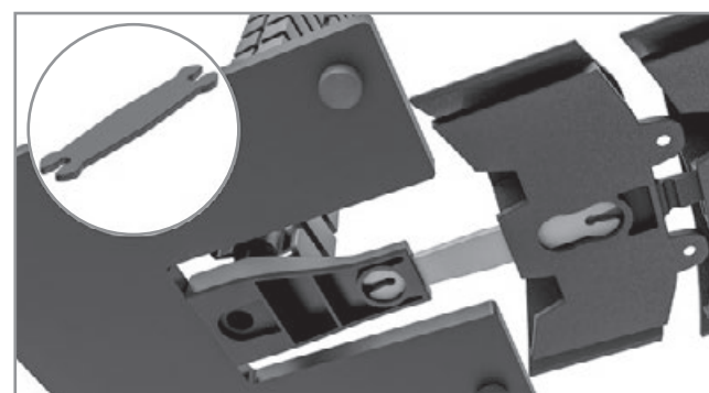
Adapter Fußplatte Adapater base plate
